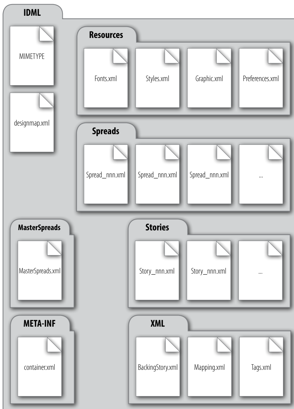
Figure 1. IDML Package Contents
