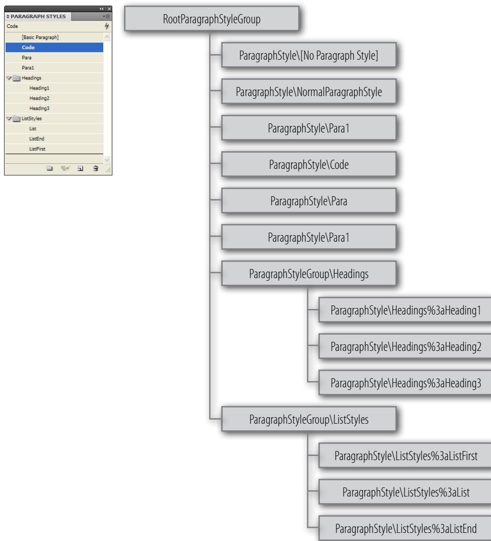
Figure 56. Example RootParagraphStyleGroup , ParagraphStyle , and ParagraphStyleGroup Elements (Self attribute values shown)
