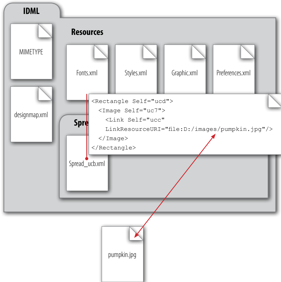
Figure 5. Cross Reference: Referring to an External File
