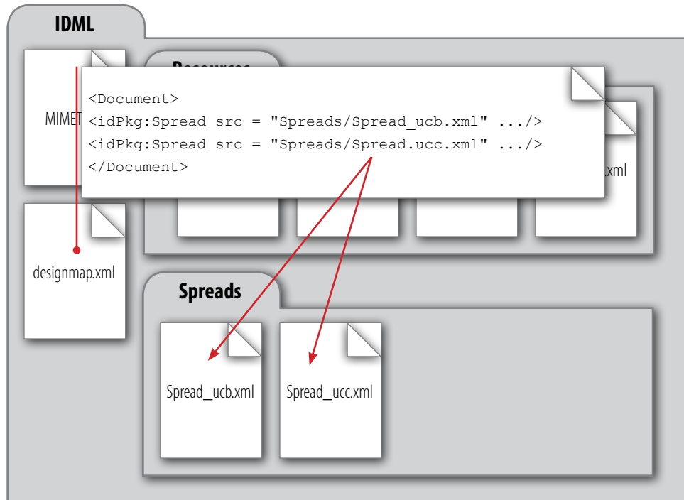
Figure 2. Cross Reference: <Document> to Spread file
