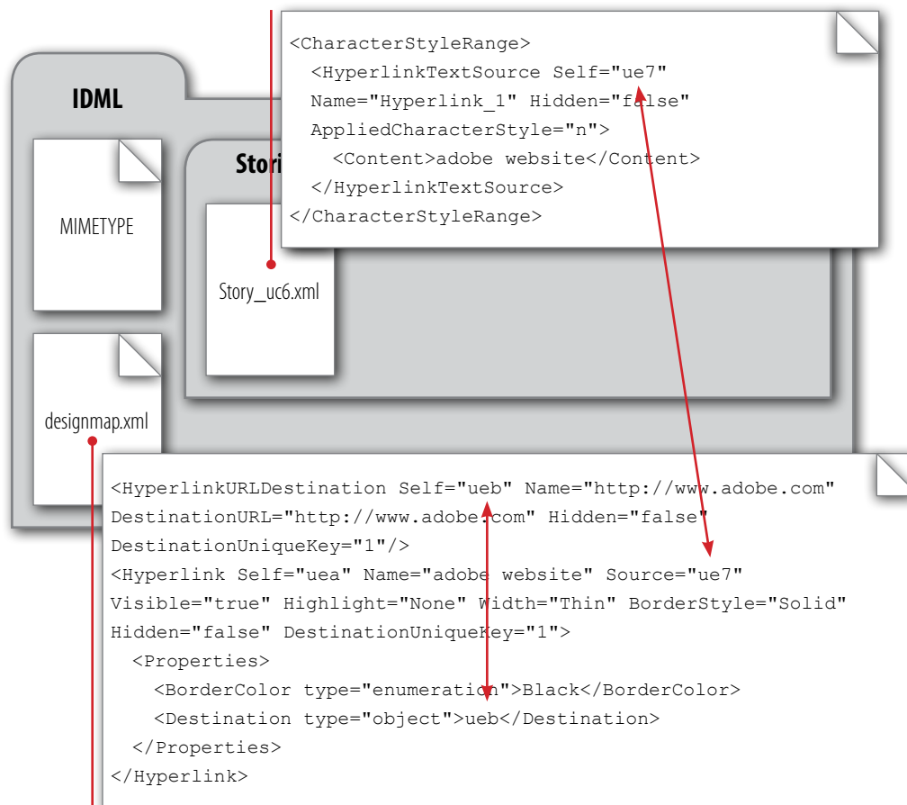
Figure 6. Cross Reference: Hyperlink Source and Hyperlink Destination
