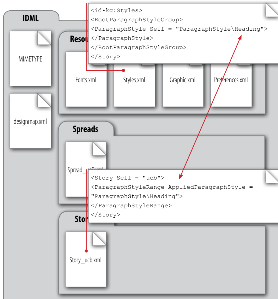
Figure 4. Cross Reference: &lt;ParagraphStyleRange&gt; to &lt;ParagraphStyle&gt;
