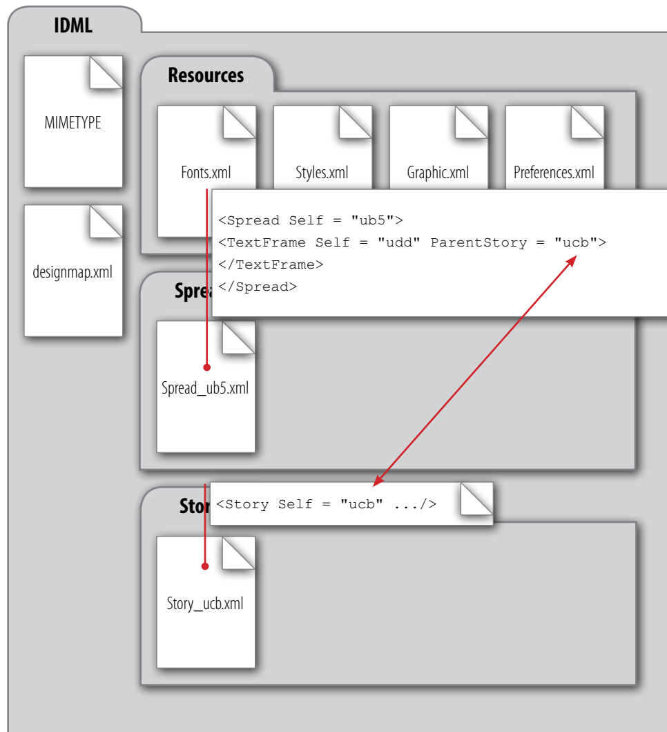
Figure 3. Cross Reference: <TextFrame> to <Story>
