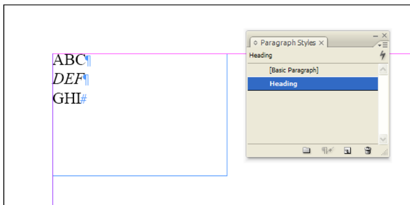
Figure 34. Minimal Story with Multiple <ParagraphStyleRange> Elements
