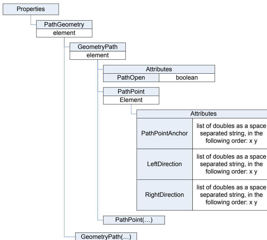
Figure 8. PathGeometry Element
