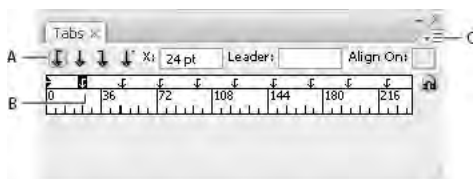
Repeated tabs
