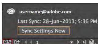
Sync status
