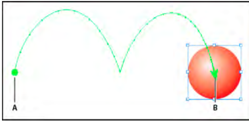
Motion path
