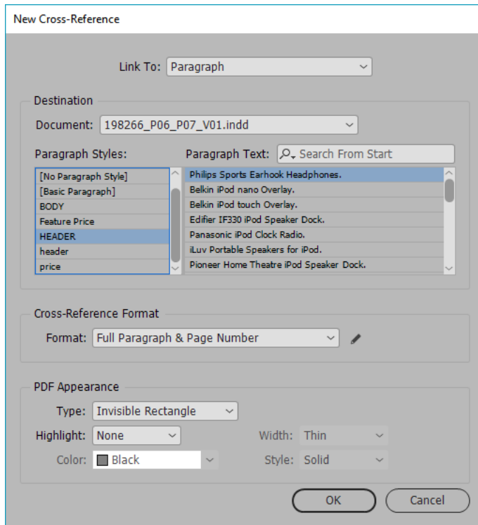
Inserting cross-references
