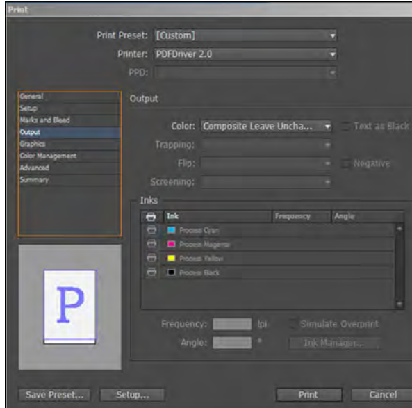
Print dialog
