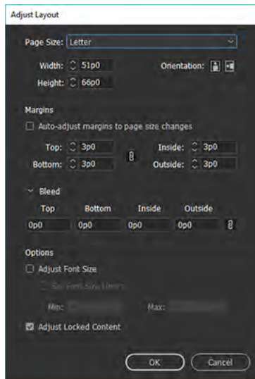
Adjust Layout
