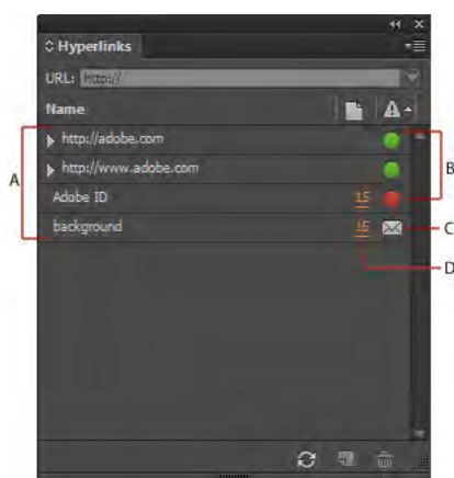
Hyperlinks panel
