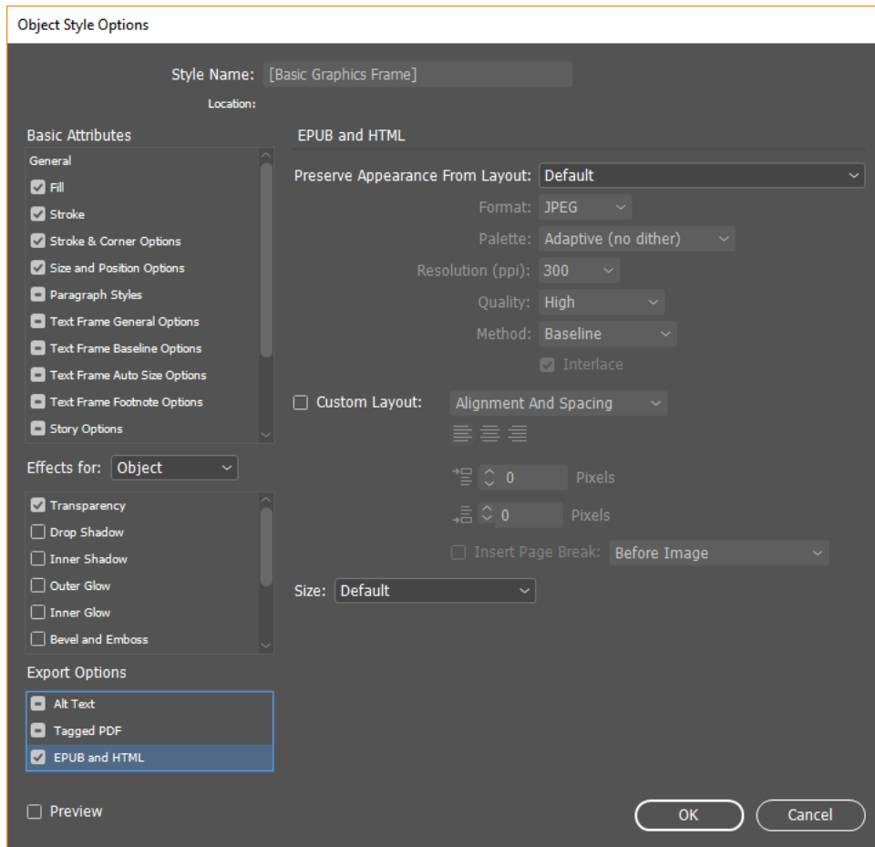
Export options
