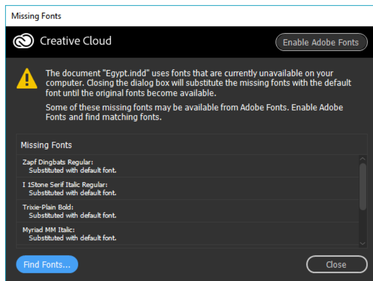
Missing fonts
